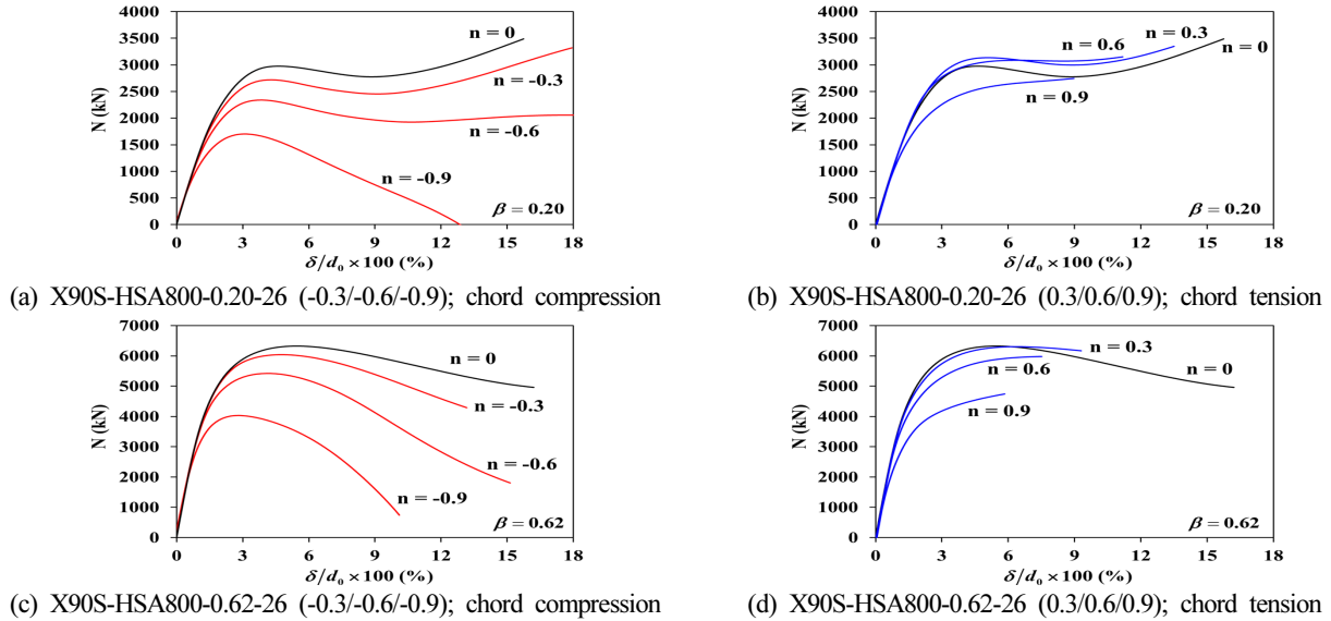
Fig. 9. Load versus out-of-plane deformation diagram for joints with chord pre-stress
