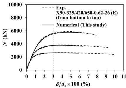
Fig. 2. Validation of numerical modeling scheme
