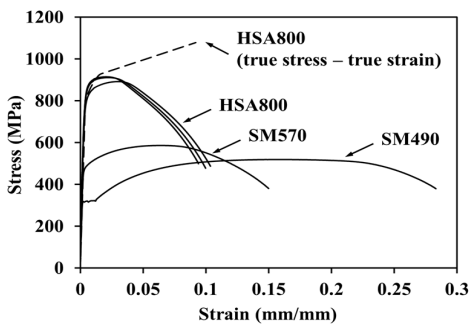
Fig. 4. Stress-strain relationship of three steel grades
