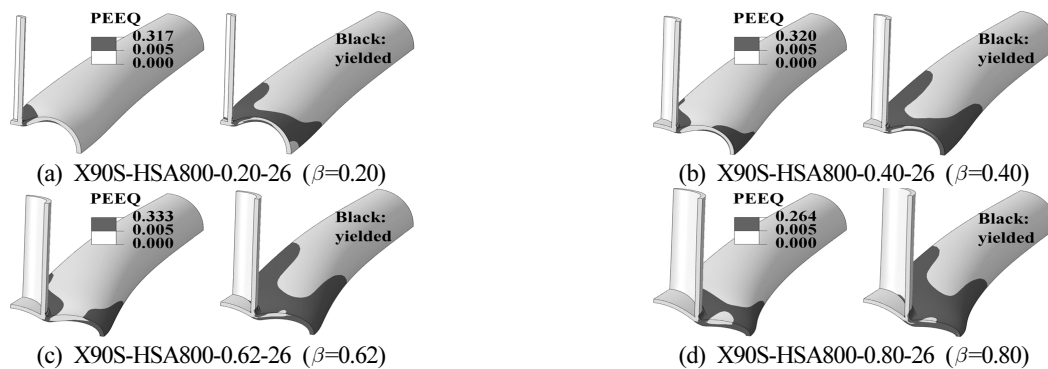
Fig. 6. Plastic equivalent strain (PEEQ, left of each) and yielded region (right of each) at peak (deformation exaggerated)
