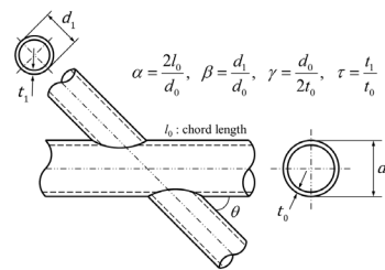
Fig. 1. General configuration and definition of symbols of CHS X-joints
