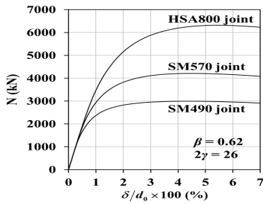
Fig. 8. Effect of steel grade on behavior of CHS X-joints
