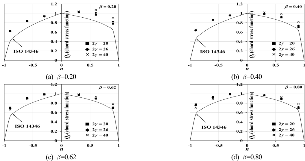
Fig. 11. Chord stress effect of HSA800 joints
