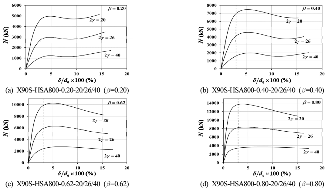
Fig. 7. Load versus out-of-plane deformation relationship of HSA800 joints
