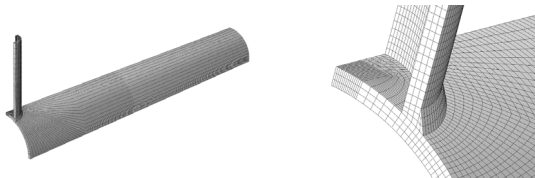
(a) overall view (b) close-up view around the joint
