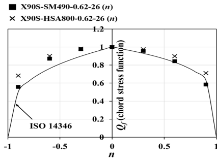
Fig. 12. Comparison of chord stress effect of SM490 and HSA800 joint
