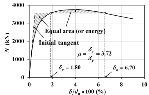
Fig. 5. Definition of joint ductility
