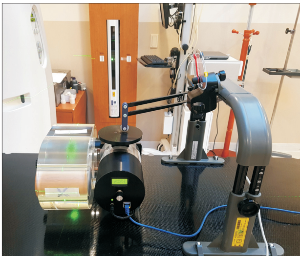
Fig. 1. The setup of QUSAR phantom and Abches system for acquiring the motion signal.
