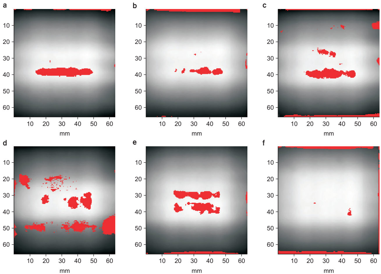
Fig. 6. 2D gamma index map (a) 5.0 s period, 1.0 cm field width; (b) 4.0 mm period, 1.0 cm field width; (c) 5.0 s period, 2.5 cm field width; (d) 4.0 mm period, 2.5 cm field width; (e) 5.0 s period, 5.0 cm field width; (f) 4.0 mm period, 5.0 cm field width; Red (dark): Gamma index >1.
