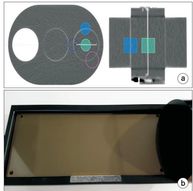
Fig. 2. (a) Target 1 and Target 2 of 3.0 cm diameter and 6.0 cm length in a QUASAR ™ phantom film cassette and Organs at Risk (OARs); (b) EBT3 film inserted in film cassette.
