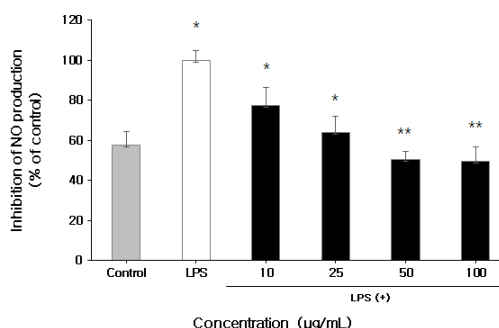
Fig. 4. Inhibition of nitric oxide production in RAW 264.7 cell treated with Psidium guajava leaf extract. The results are presented as the mean \pm S.D. of three independent experiments (* p <.05, ** p <.01).
