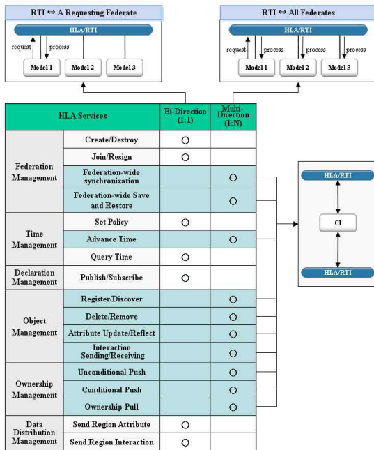
Fig. 3. HLA service relaying through CI
