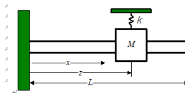
Fig. 1. Schematic diagram of the clamped-free beam with the added mass at x=z(=\zeta L) .
