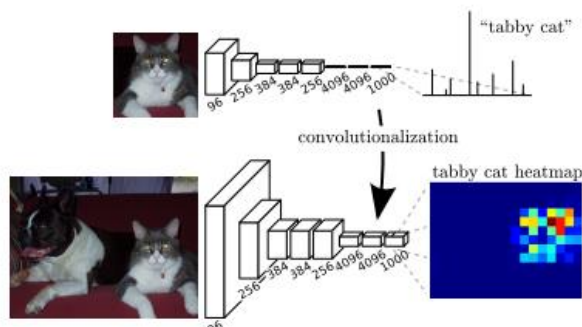
Fig. 2. Transforming fully connected layers into convolution layers enables a classification net to output a heat map. Adding layers and a spatial loss produces an efficient machine for end-to-end dense learning [26].
