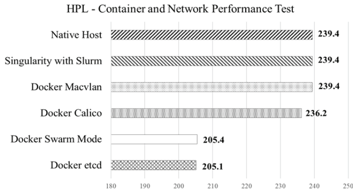
Fig. 2. Performance test with HPL benchmark.
