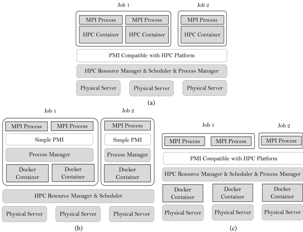
Fig. 1. HPC platform structure. (a) HPC container integration with existing HPC platform. (b) Docker case 1: container as MPI process of each job. (c) Docker case 2: container as HPC worker node.
