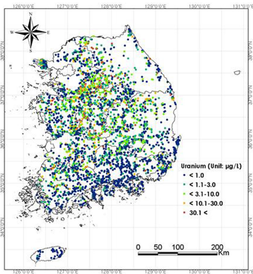
Fig. 3. Spatial distribution of uranium concentrations from 3,820 CGS groundwaters.
