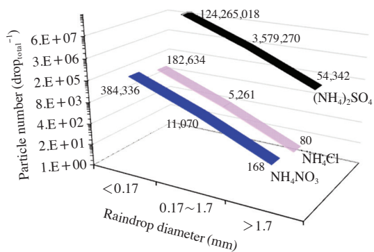
Fig. 5. Theoretically calculated particle number of three kinds of secondary particles scavenged in three-step of raindrop size spectra.
