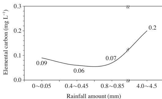
Fig. 4. Variation of elemental carbon in rainwater as a function of rainfall amount.
