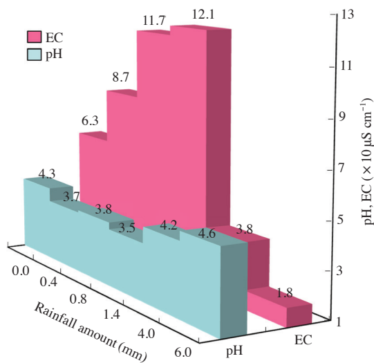
Fig. 2. Variation of pH and electrical conductivity (EC) of bulk rainwater as a function of rainfall amount.
