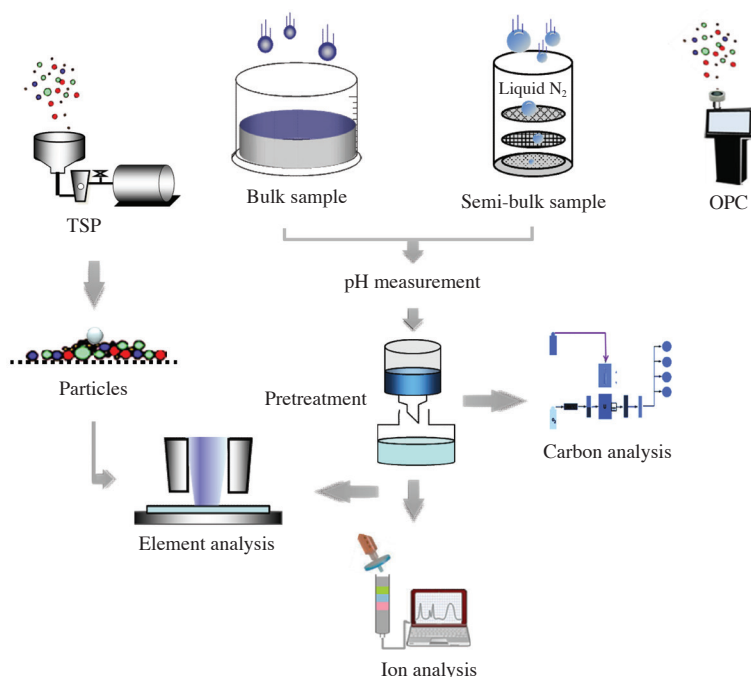
Fig. 1. Flow of sampling, pretreatment, and analysis of bulk and semi-bulk rain samples.
