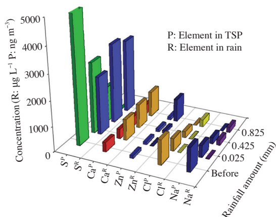
Fig. 3. Variation of several interested elements in TSP and bulk rain samples collected before and during an initial rainfall event.
