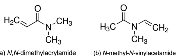
(a) N,N -dimethylacrylamide (b) N -methyl- N -vinylacetamide Figure 1. Structures of additives [(a): DMA, (b): NMV].
