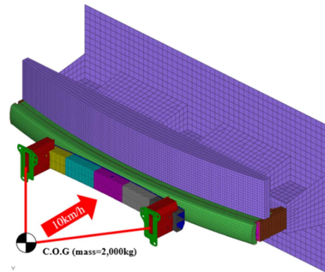
Fig. 1. IIHS bumper crash analysis (Full overlap)
