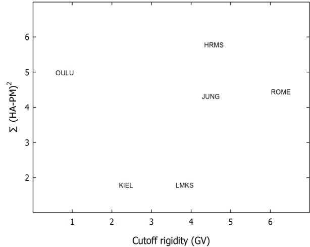
Fig. 6. Variance in maximum phase between harmonic analysis method and pile-up method for the six neutron monitors.
