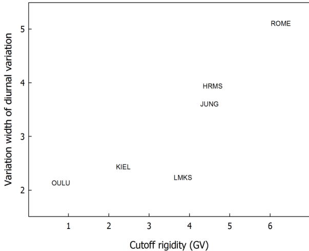
Fig. 5. Variation width of diurnal variation related to the solar cyclic modulation by harmonic analysis at six neutron monitors.
