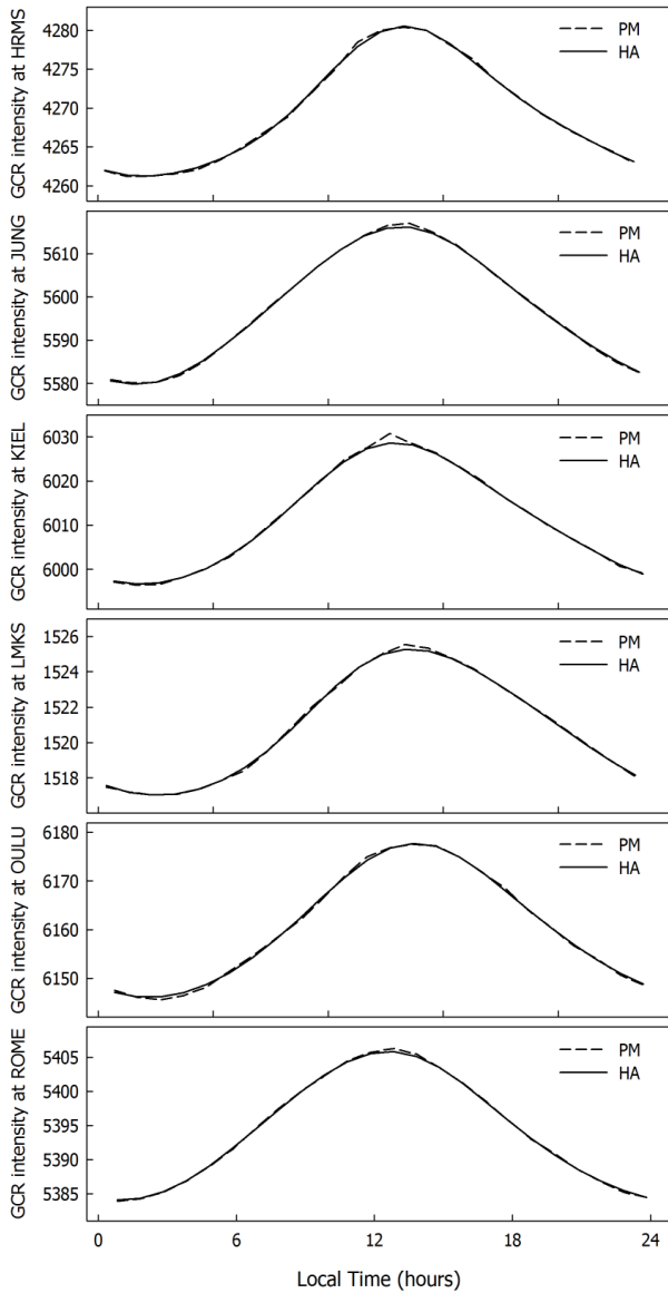
Fig. 1. Diurnal variation in the entire analyzed period at the six neutron monitors (from top to bottom: Hermanus, Jungfrauoch, Kiel, Lomnicky Stit, Oulu, and Rome). The dashed and solid lines represent the diurnal variation by pile-up method and harmonic analysis, respectively.
