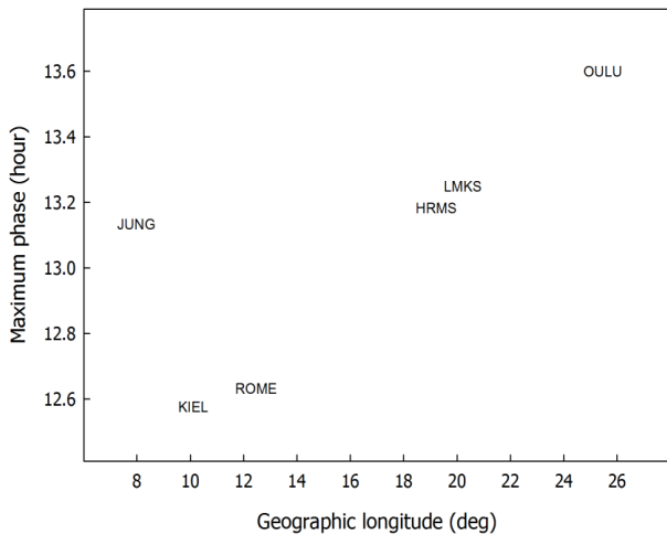
Fig. 2. Maximum phase by harmonic analysis in relation to the longitude of the neutron monitor for the entire analyzed period shown in Fig. 1. Names indicate the neutron monitor station code shown in Table 1.
