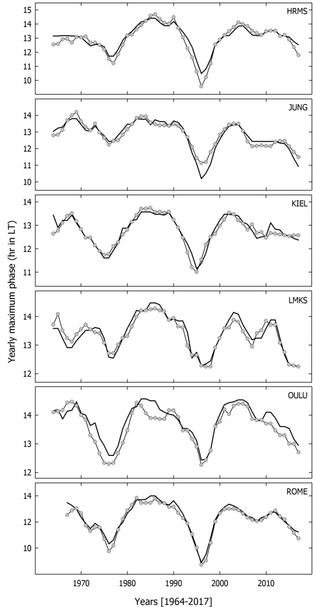
Fig. 4. Solar cyclic modulation of maximum phase at six neutron monitors. The labels indicate the neutron monitor station code. The solid line and line with circles indicate the maximum phase by harmonic analysis and by pile-up method, respectively.
