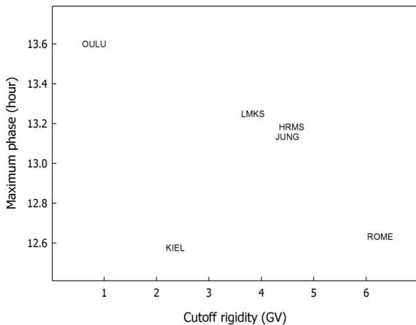
Fig. 3. Maximum phase by harmonic analysis in relation to the cutoff rigidity of the neutron monitor for the entire analyzed period shown in Fig. 1. The display is the same as in Fig. 2.
