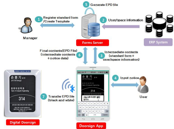
Fig. 5. System Configuration[11]
