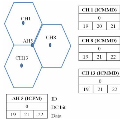
Fig. 9. ICFM list calculation
