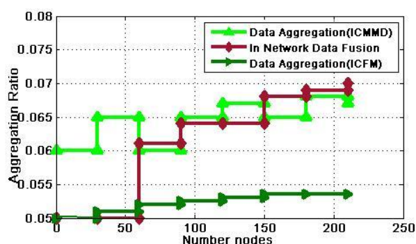
Fig. 15. Aggregation Ratio
