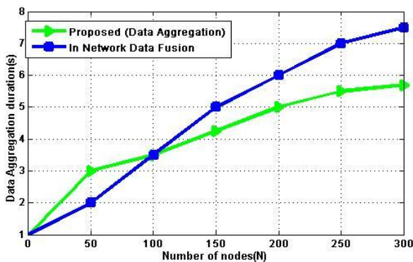
Fig. 12. Data aggregation duration
