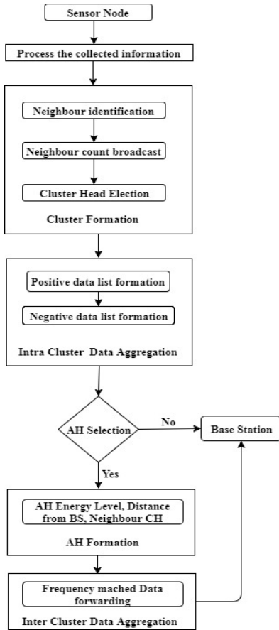
Fig. 2. Flow diagram of the proposed system
