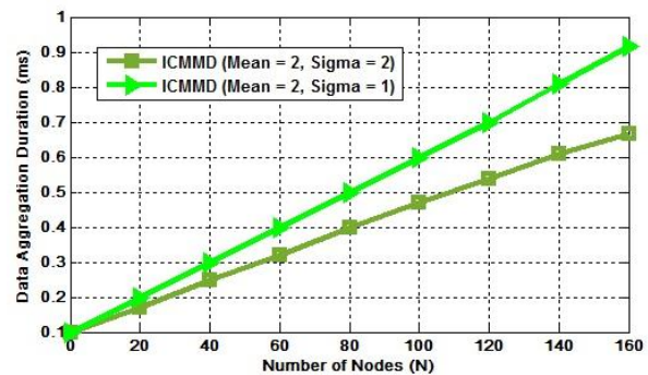
Fig. 13. Data aggregation duration with difference variance of ICMMMD
