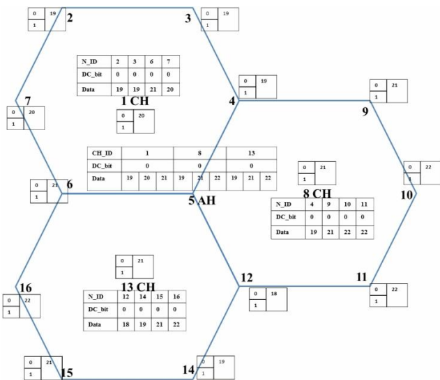
Fig. 7. Intra cluster data aggregation
