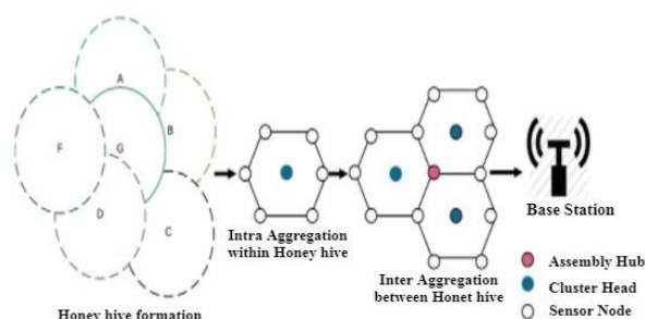
Fig. 1. Proposed Architecture
