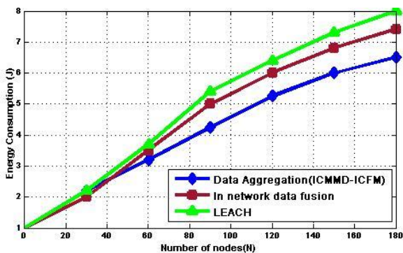
Fig. 11. Energy consumption according to the number of iterations
