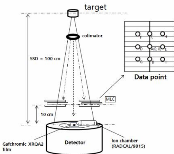
Fig. 3. Experimental Setup for evaluation of utility of the diagnostic multi-leaf collimator with ion chamber (Data point refer to measurement point using ion chamber)
