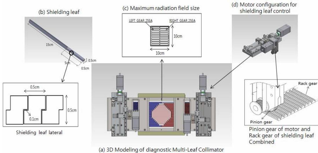
Fig. 1. Engineering design of diagnostic multi-leaf collimator
