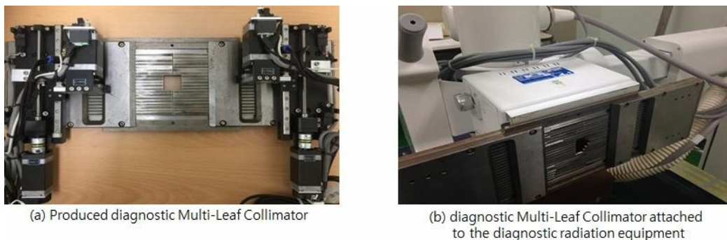
Fig. 2. Produced diagnostic multi-leaf collimator and attach the diagnostic radiation equipment
