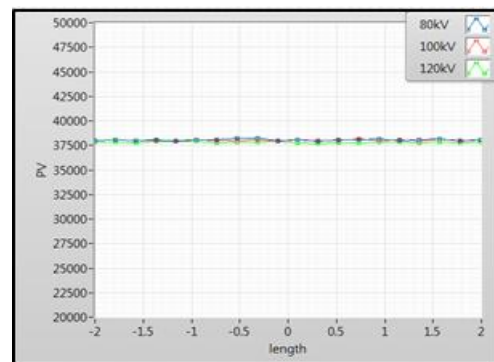
(b) Dose distribution between longitudinal leaves in MLC field (Y-axis)
