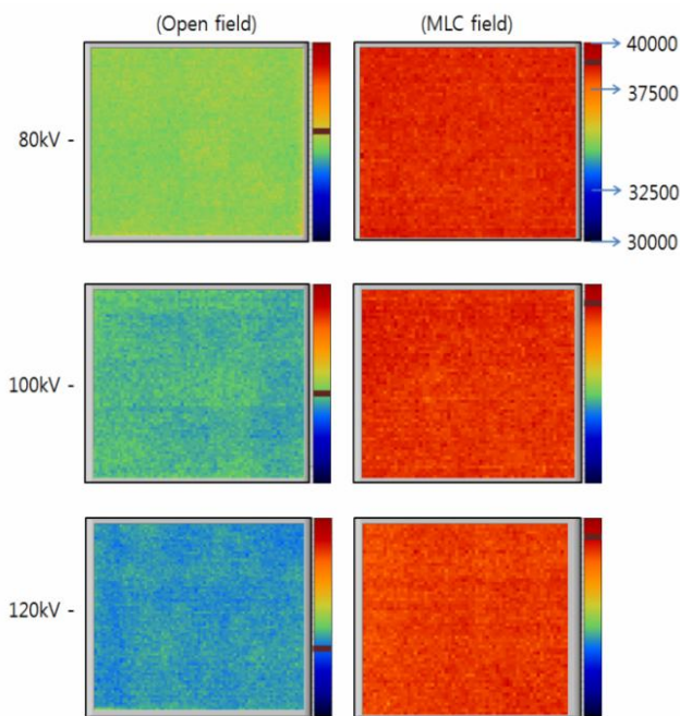
Fig. 6. Color Mapping of Dose Distribution resulted from the diagnostic Multi-leaf Collimator (Open field and MLC field)
