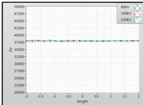
(a) Dose distribution between longitudinal leaves in MLC field (X-axis)
