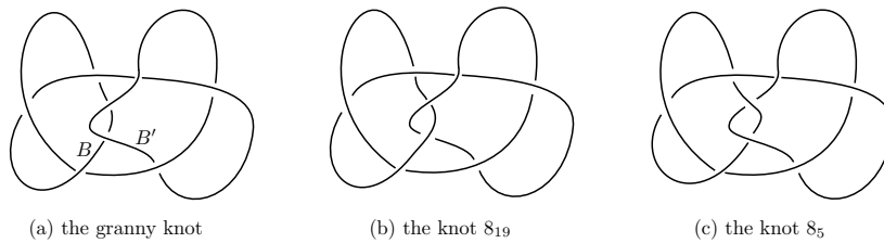
FIGURE 8. R-related diagrams: the granny knot, 8_{19} , and 8_5 .
