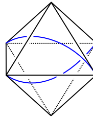
(b) 5-term triangulation
