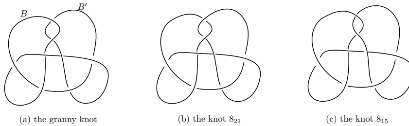
FIGURE 7. R-related diagrams: the granny knot, 8_{21} , and 8_{15} .
