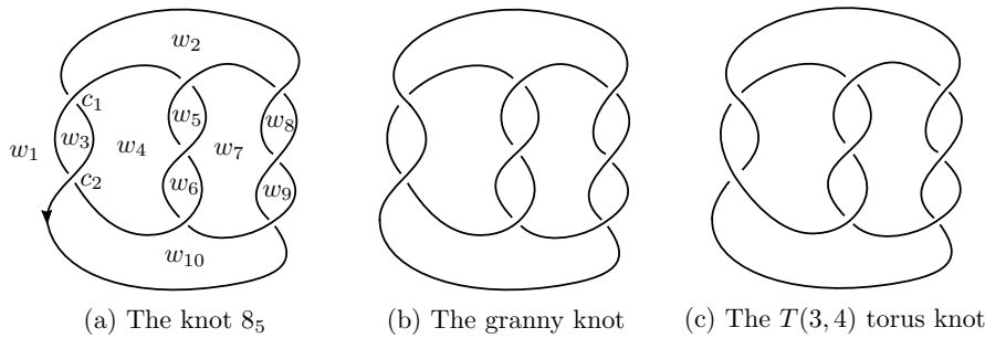
FIGURE 4. The 8_5 knot diagram and R -related diagrams.
