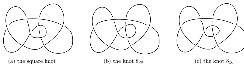
FIGURE 9. R-related diagrams: the square knot, 8_{20} , and 8_{10} .
