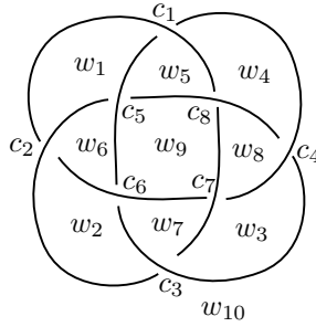
FIGURE 5. The 8_{18} knot diagram.
