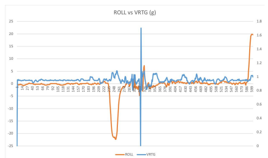
Fig 5. Roll vs Vertical G
