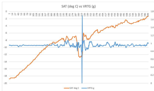
Fig 6. SAT vs Vertical G
