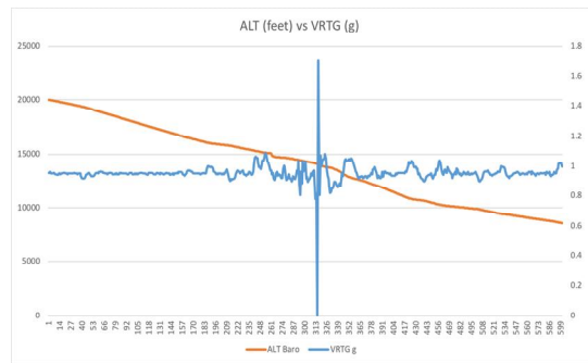
Fig 3. ALT vs Vertical G
