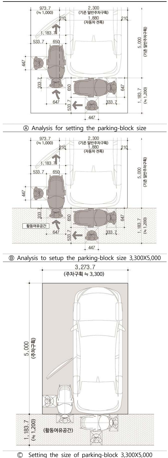
[Figure 12] Analyzing and Setting for Parking-Block Size(mm)
