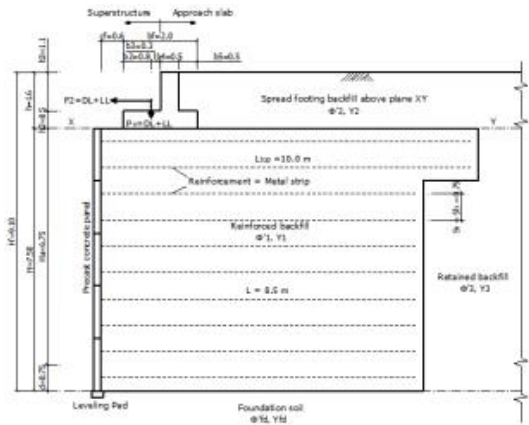
Fig. 4. Cross Sectional View of MSEW abutment
