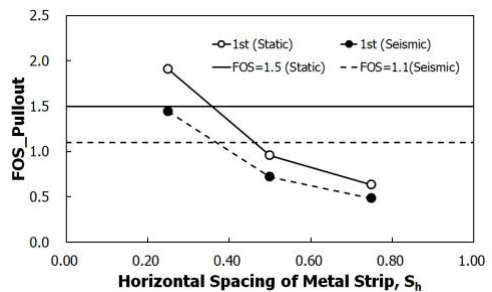
Fig. 8. Pullout Safety Factors by variation of reinforcement spacing
