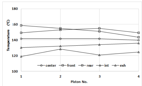
Fig. 7. Temperature of Piston Head with Oil Jet
