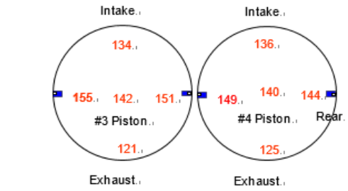
Fig. 5. Temperature of Piston Head with Oil Jet
