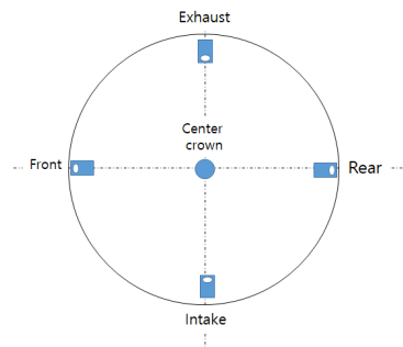
Fig. 2. Templug Location in Piston
