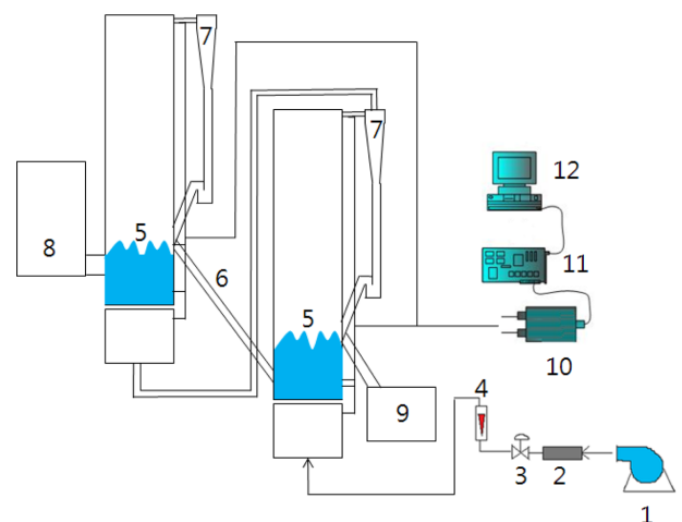
Fig. 1. Two-stage fluidized-bed system.
