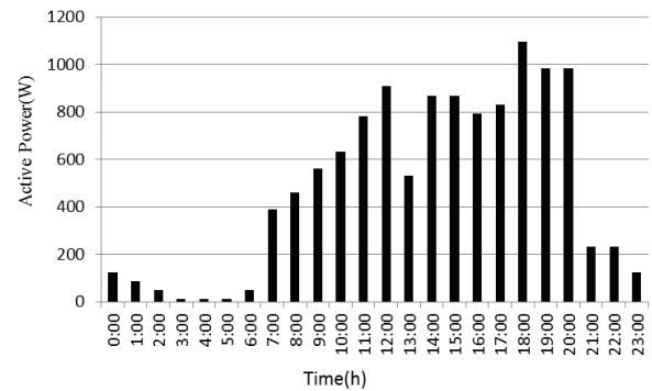
Fig. 4. Active power of non-thermal loads
