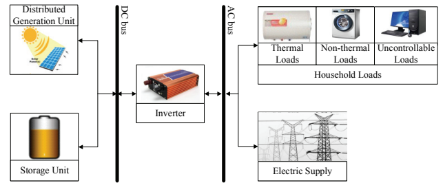
Fig. 1. The structure of a typical residential house
