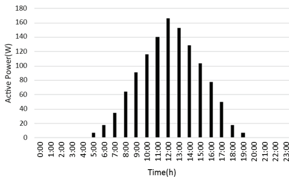
Fig. 3. Power of the photovoltaic array
