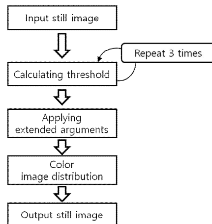
Fig. 4. Proposed algorithm's total flowchart.
