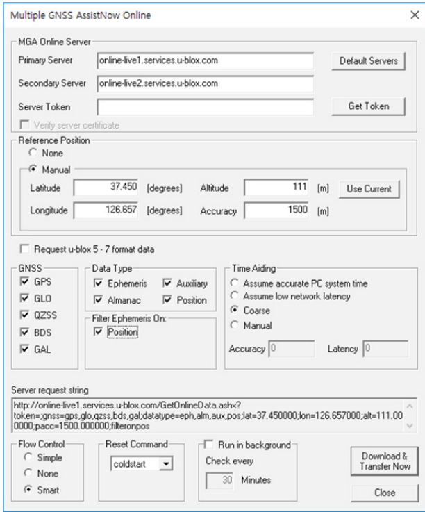
Fig. 6. The GUI of AssistNow online.
