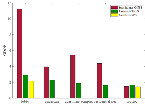
Fig. 9. Comparison of GDOP for each scenario; Standalone-GNSS vs. A-GPS vs. A-GNSS.
