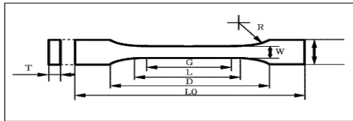
W: 3 mm, G: 9 mm, L: 12 mm, D: 25 mm, L0: 63 mm, R: 6 mm, T: 3 mm
