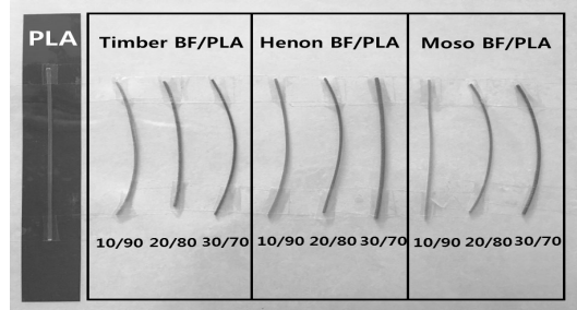
Fig. 6. BF/PLA filament by content of bamboo flour.
