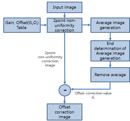
Fig. 5. Functional flow chart of general non-uniformity correction method
