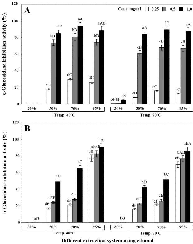
Fig. 4. Comparison of \alpha -glucosidase inhibition activity on extracted Genuderma lucidum of two fruiting bodies from different extract system of ethanol.
