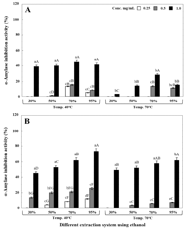
Fig. 5. Comparison of \alpha -amylase inhibition activity on extracted Genuderma lucidum of two fruiting bodies from different extract system of ethanol.
