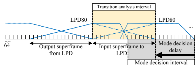
Fig. 4. Transition analysis interval with the LPD extension.
