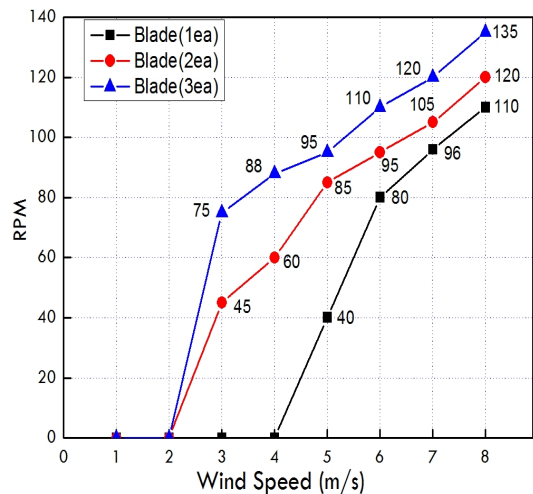
Fig. 4. Generator RPM according to wind speed
