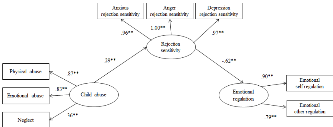
Fig. 4. Structural model
