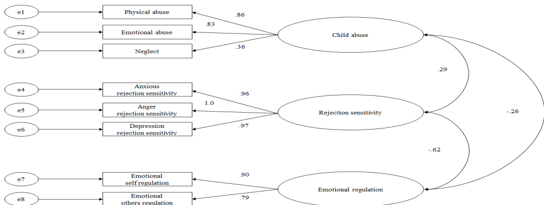
Fig. 3. Measurement model
