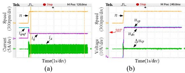
Fig. 11. Measured transient performance of the drive of the proposed control scheme during the starting process: (a) rotor speed, q -axis current and phase-A current; (b) rotor speed, DC capacitor voltages and voltage difference between the upper and lower capacitors in the DC link.
