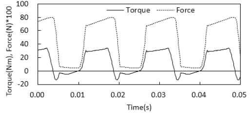
(e) Torque on cam and force on bucket tappet
