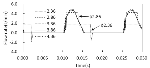
(a) Inlet valve flow rate
