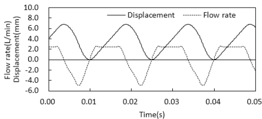
(a) Plunger disp. and pumping chamber flow rate
