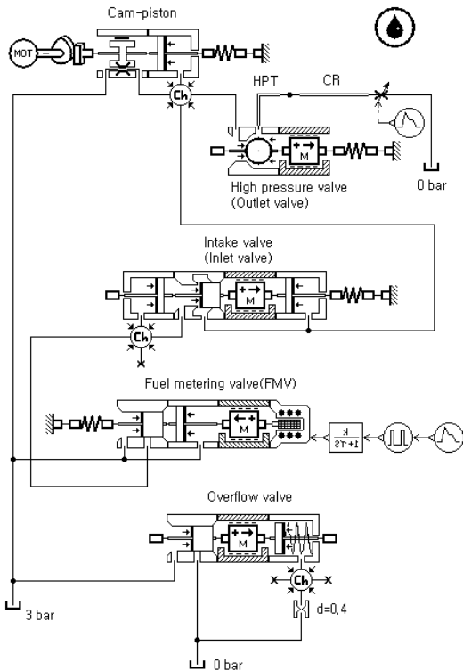
Fig. 8. Simulation model of high pressure pump
