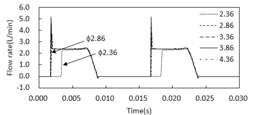
(b) Outlet valve flow rate
