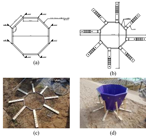
Fig. 1. Drawing of hydraulic well (a)18mm Octagon stainless steel (b)Lower bracket (c)Lower bracket installation view (d)Finished goods
