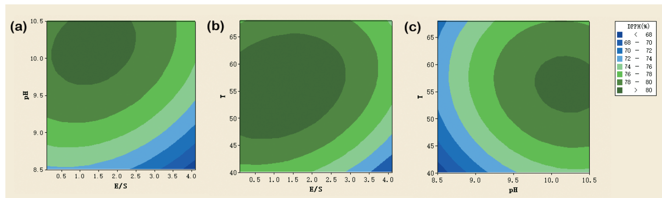
Figure 1. Contour plots of 1,1-diphenyl-2-picrylhydrazyl radical scavenging activity as functions of (a) enzyme-to-substrate ( E/S ) ratio vs pH at temperature of 54°C, (b) E/S ratio vs temperature at pH of 9.5, and (c) pH vs temperature at an E/S ratio of 2.1%.
