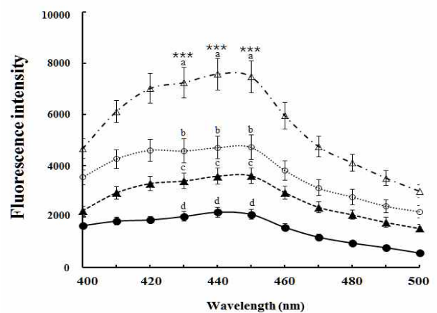
Fig. 3. Fluorescence spectra (excitation=360 nm) in organic phase of chloroform/methanol extractions (***) p<0.0001 .
