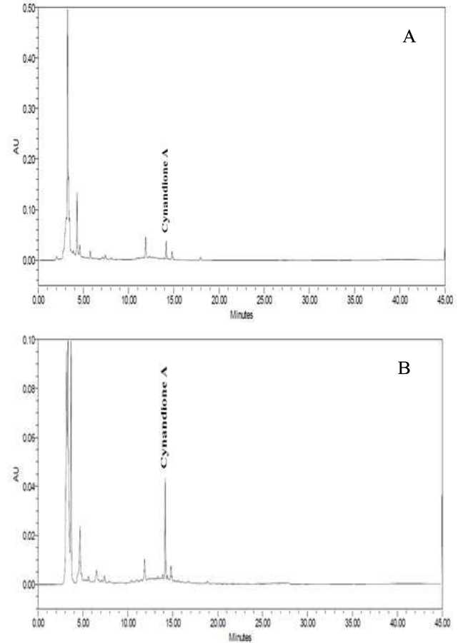
Fig. 1. HPLC chromatograms of Cynanchi wilfordii Radix extracts.
