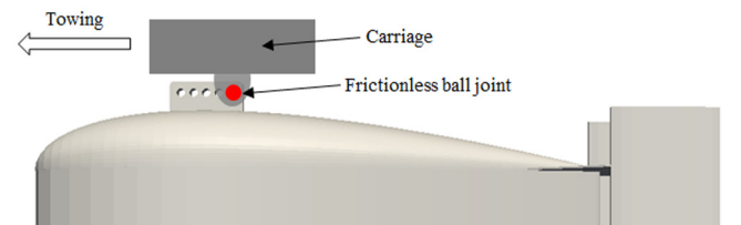
Fig. 3 Boundary conditions of towing point
