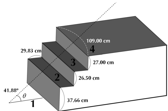
Figure 1. Structure of bus stair
