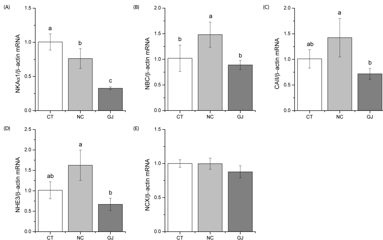
Fig. 5. Sodium transporter gene expression in kidney cortex. Values are shown as the means \pm SD. Values with different letters within a column are significantly different from each other at P < 0.05 by Duncan's multiple range test ( a > b > c ). CT, Control; NC, NaCl group; GJ, ganjang group. NKA \alpha 1, Na ^+ /K ^+ ATPase \alpha 1; NBC, Na ^+ /HCO _3^- co-exchanger; CAII, carbonic anhydrases II; NHE3, Na ^+ /H ^+ exchanger 3; NCX, Na ^+ /Ca ^{2+} exchanger.
