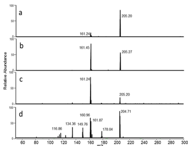
Figure 2. Collisionally induced dissociation spectra of [M-H]^+ ions of ibuprofen depended on various collision energy. a: 5 eV, b: 8 eV, c: 10 eV, d: 15 eV.
