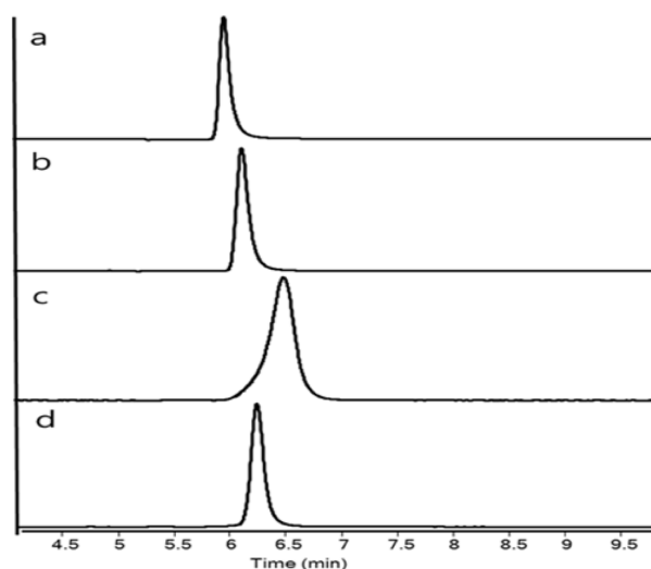
Figure 1. SIM chromatograms of ibuprofen observed from different compositions of 10 mmol/L ammonium acetate and organic solvent. a: Acetonitrile (90%, v/v), b: Acetonitrile (80%, v/v), c: Methanol (90%, v/v), d: Acetonitrile:Methanol (1:1, 90%, v/v).
