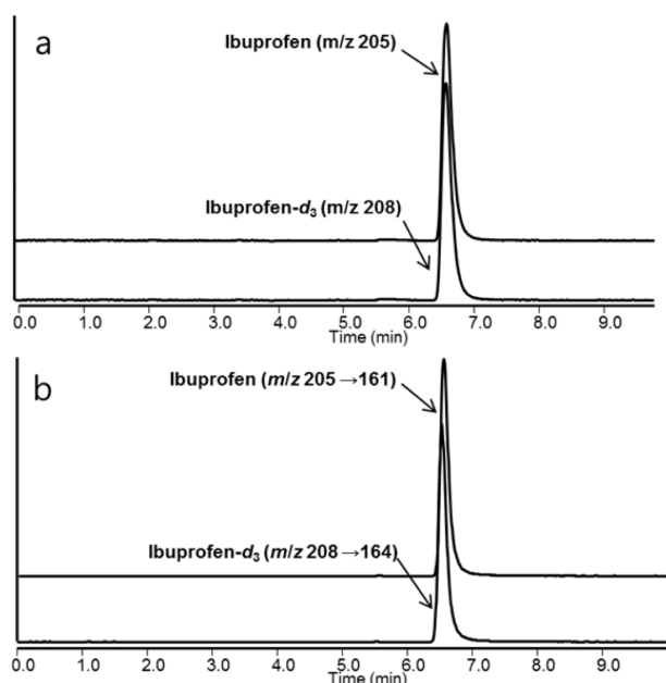
Figure 3. SIM (a) and SRM (b) chromatograms of ibuprofen and ibuprofen- d_3 in homogenized analgesic tablets.
