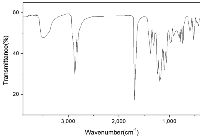
Fig. 1. FT-IR spectrum of synthesized ARAA-6-20.
