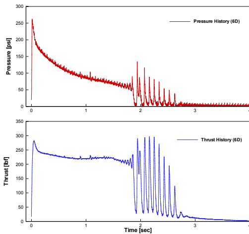
Fig. 8 Pressure/Thrust history for nozzleless booster at L/D=6.
