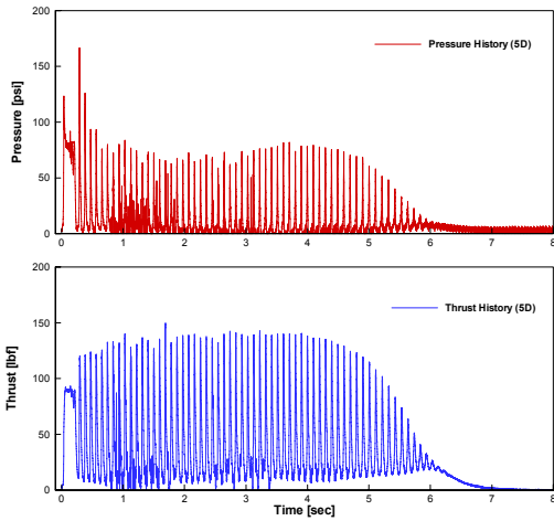
Fig. 7 Pressure/Thrust history for nozzleless booster at L/D=5.
