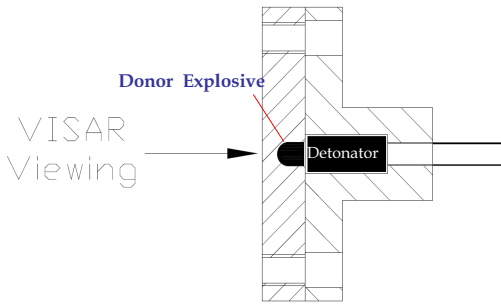
Fig. 2 TBI for VISAR experiment.
