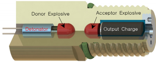
Fig. 1 Through-bulkhead initiator.
