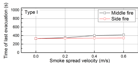
(h) Type I of island platform
