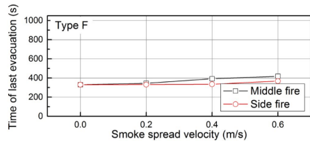
(b) Type F of island platform
