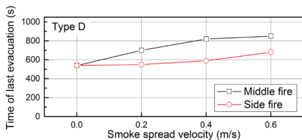
(g) Type D of side platform
