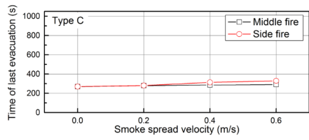
(e) Type C of side platform
