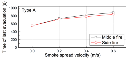
(a) Type A of side platform
