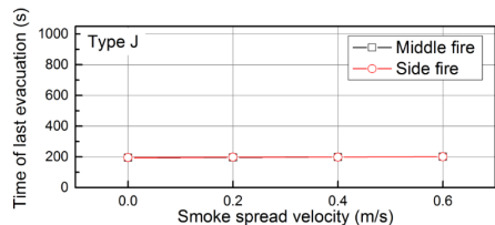
(j) Type J of island platform
