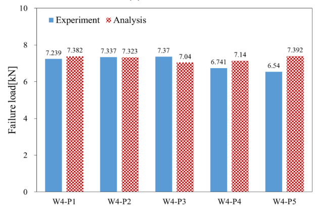
(b) Yamada-Sun
