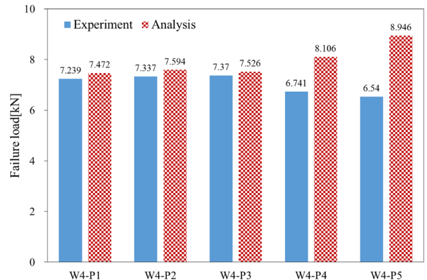
(a) Tsai-Wu
