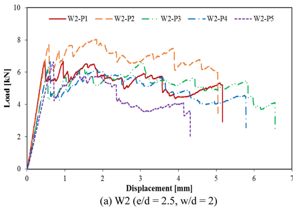
Fig. 4. Tensile test of the composite joint specimen
