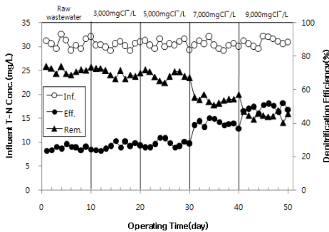
Fig. 9. Comparison of the T-N concentration according to salt concentration in continuous reactor.
