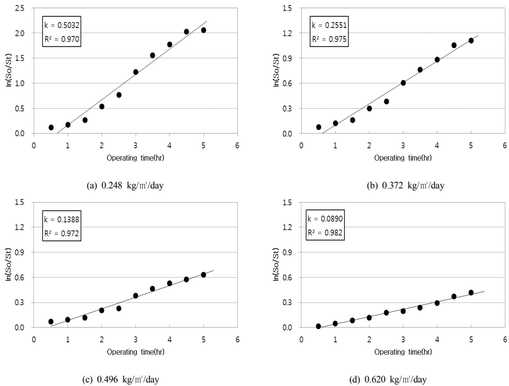
Fig. 6. Graphical determination of the decay rate coefficients due to VLR(T-N).
