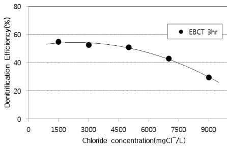
Fig. 8. Variation of denitrification efficiency with various salt concentration in batch-reactor.
