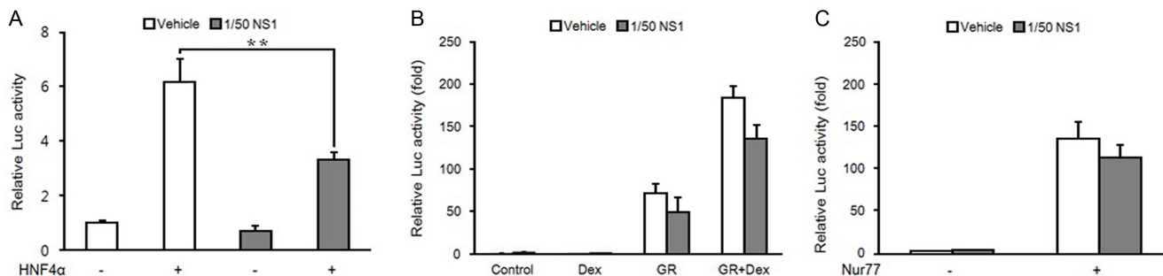
Fig. 3. LNS1-CM specifically inhibits HNF4α transcriptional activity in HepG2 cells. (A)-(C) HEK293T cells were transfected with a luciferase reporter plasmid linked to the PEPCK promoter spanning -472 to +79 (pGL3-PEPCK-Luc, 300ng) and expression plasmids for the different transcription factors (HNF4α, GR or Nur77, each 100 ng of each) as indicated. After 12 h transfection, cells were incubated with bacterial culture media (vehicle) or LNS1-CM in the presence or absence of ligand (250 nM Dexamethasone for GR) for 24 h and then assayed for luciferase activity. ** p <0.01.
