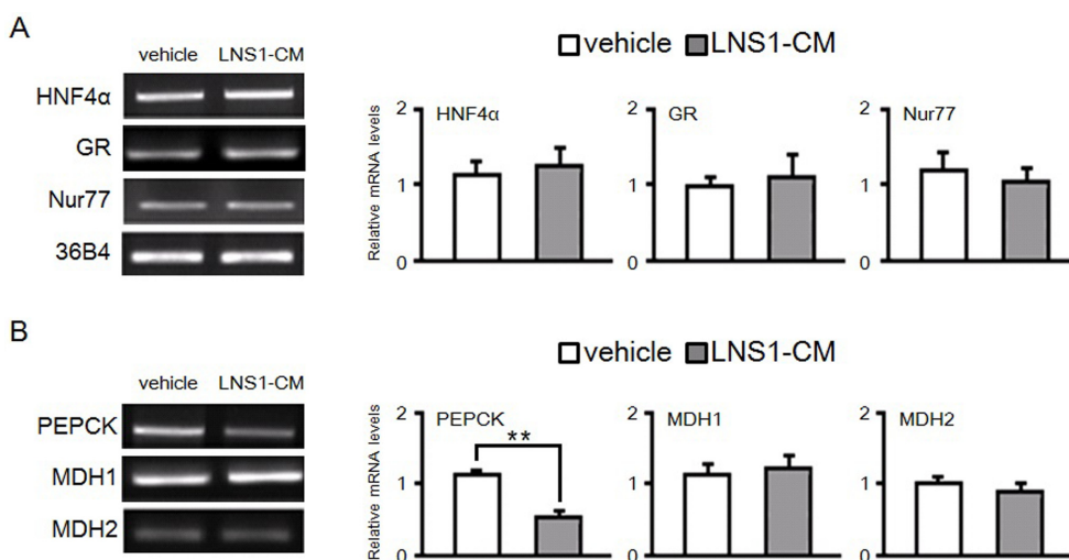
Fig. 2. Effect of LNS1-CM on gluconeogenic gene transcription in HepG2 cells. HepG2 cells were incubated with or without LNS1-CM for 24 h. mRNA was isolated from cells and transcription levels of transcription factor genes important for glucose homeostasis (A), and enzyme genes involved in gluconeogenesis (B) were determined by RT-PCR. ** p <0.01.
