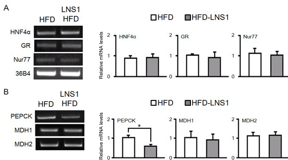
Fig. 1. LNS1 inhibits PEPCK gene transcription in liver of HFD-fed mice. Seven week-old male mice were fed a HFD with or without oral administration of LNS1 for 12 wk. mRNA was extracted from liver of each group of mice and transcription levels of transcription factor genes important for glucose homeostasis (A), and enzyme genes involved in gluconeogenesis (B) were determined by RT-PCR. * p < 0.05 .
