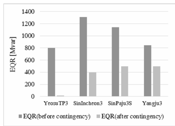
Fig. 6. EQR changes at sink areas after contingencies
