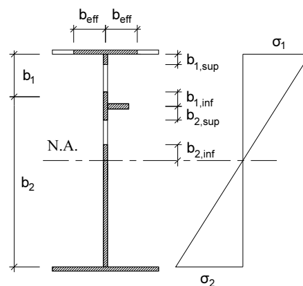
Fig. 1. Effective cross-section of girder [2]
