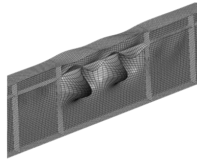
(c) Example of web-flange buckling ( b_{fc} \times t_{fc} = 500 \times 40 \text{ mm} , t_w = 10 \text{ mm} )
