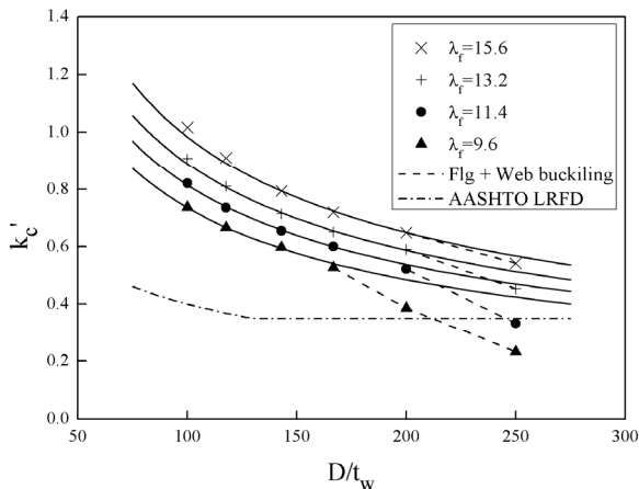
Fig. 3. Regression of flange buckling coefficients [10]
