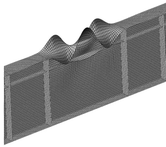
(b) Example of flange buckling ( b_{fc} \times t_{fc} = 500 \times 19 \text{ mm} , t_w = 15 \text{ mm} )
