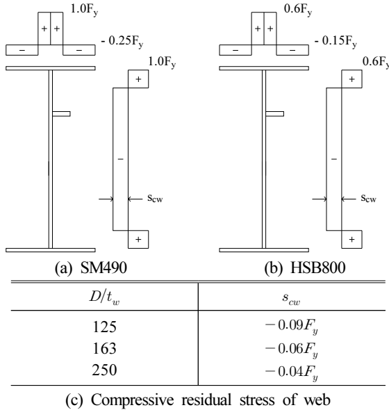
Fig. 5. Residual stress model
