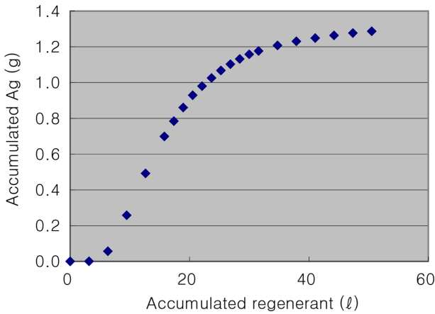
Fig. 14. Accumulated Ag quantity in effluent of backwashing process as a function of accumulated regenerant.
