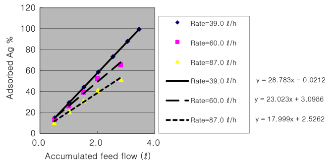
Fig. 3. The diagram of Adsorbed Ag % vs. Accumulated feed flow.
